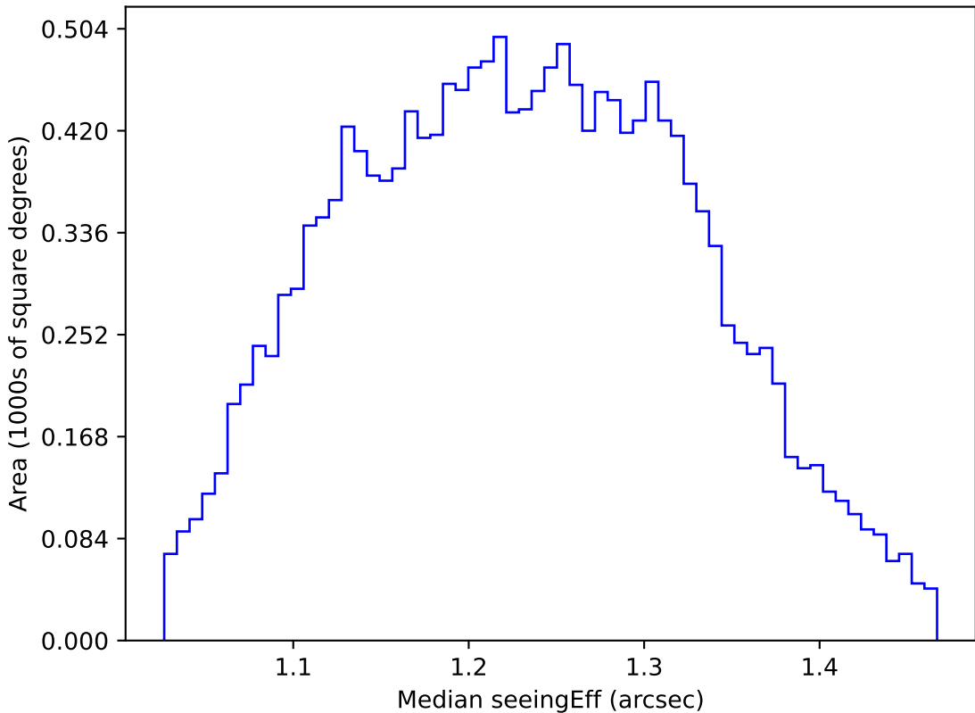
too_elab_r64_d3_giz_v3.4_10yrs WFD u band: Median seeingEff
