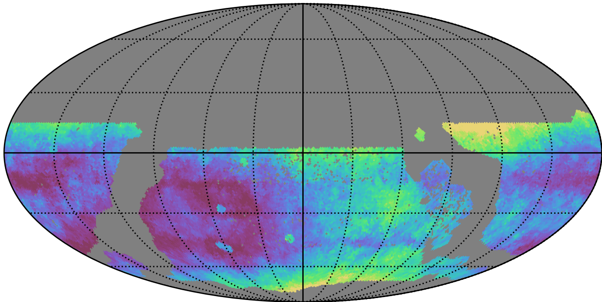
too_elab_r64_d3_giz_v3.4_10yrs WFD r band: Median seeingEff
