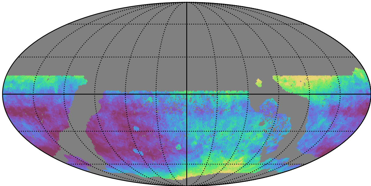
too_elab_r64_d3_giz_v3.4_10yrs WFD i band: Median seeingEff
