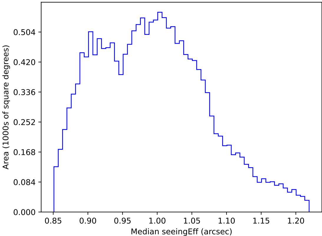
too_elab_r64_d3_giz_v3.4_10yrs WFD i band: Median seeingEff
