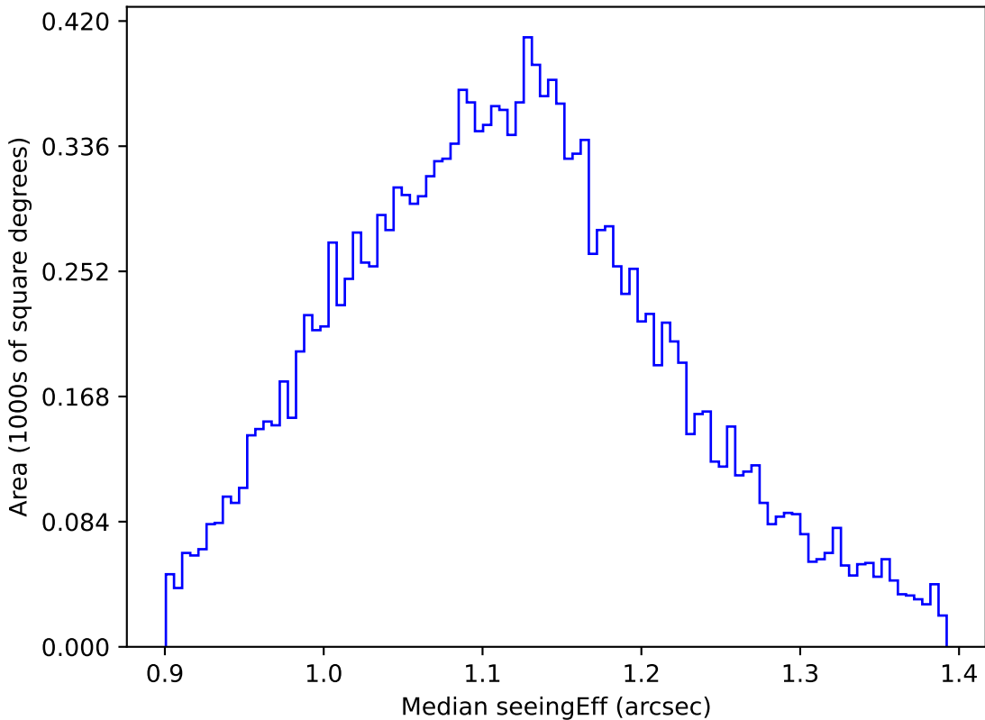
too_elab_r64_d3_giz_v3.4_10yrs WFD g band: Median seeingEff
