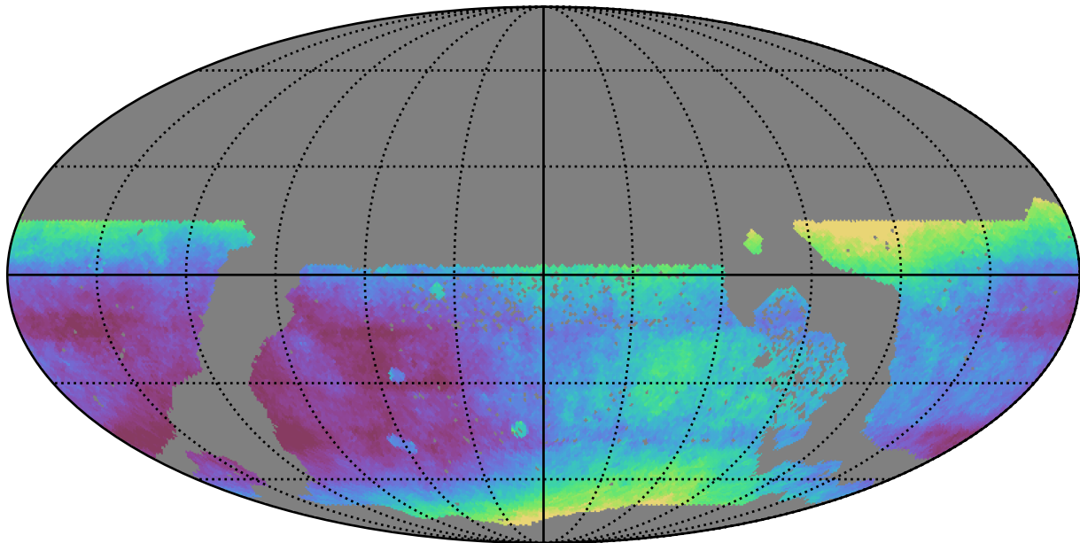
too_elab_r64_d3_giz_v3.4_10yrs WFD all bands: Median seeingEff
