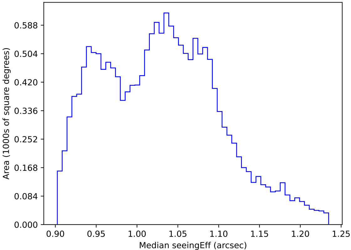
too_elab_r64_d3_giz_v3.4_10yrs WFD all bands: Median seeingEff
