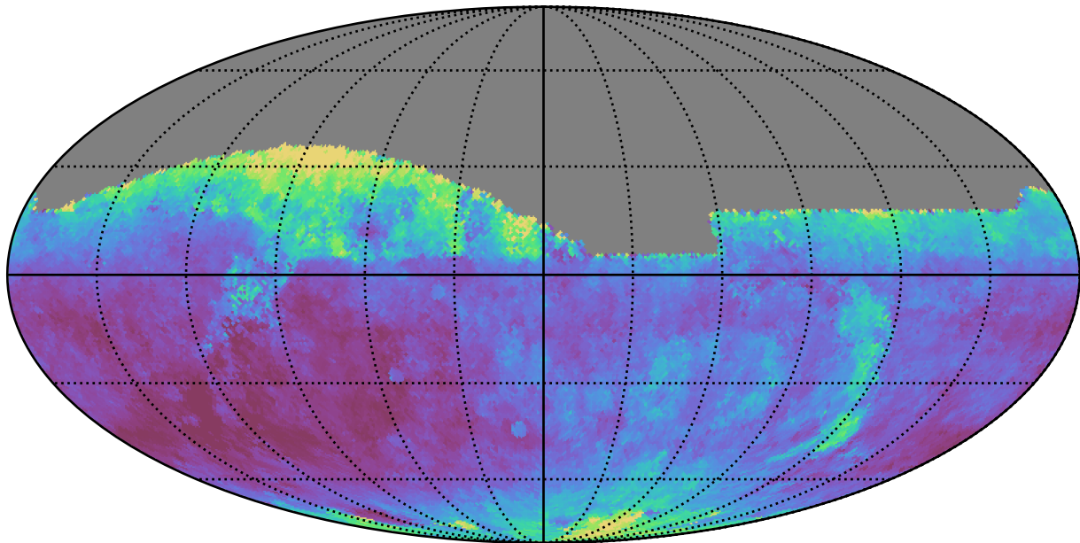
too_elab_r64_d3_giz_v3.4_10yrs All sky z band: Median seeingEff
