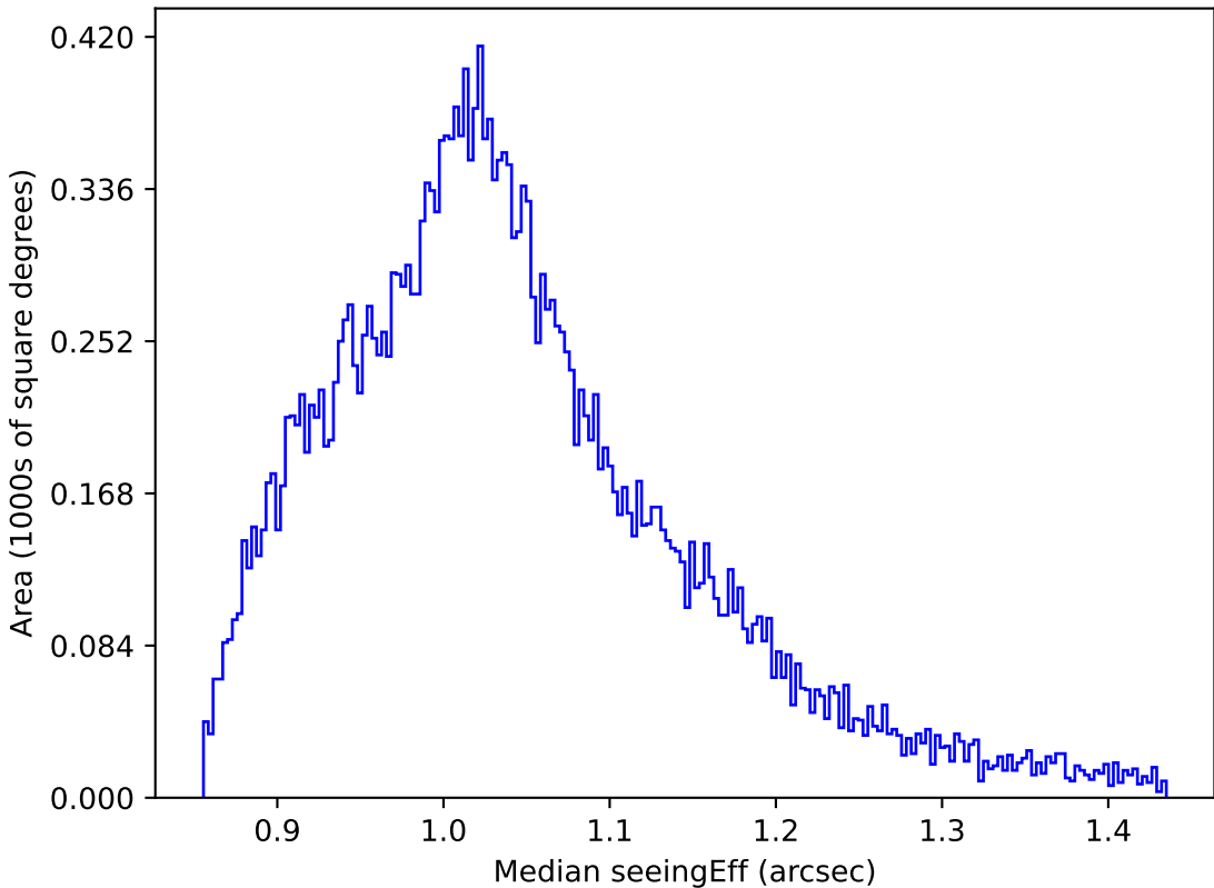
too_elab_r64_d3_giz_v3.4_10yrs All sky z band: Median seeingEff
