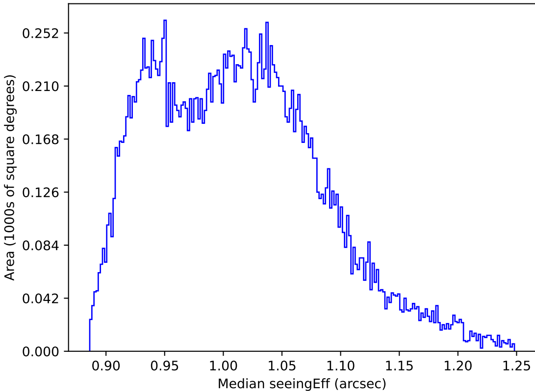
too_elab_r64_d3_giz_v3.4_10yrs All sky y band: Median seeingEff
