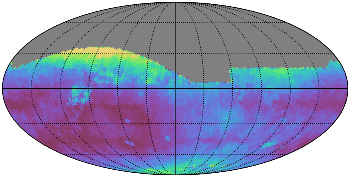
too_elab_r64_d3_giz_v3.4_10yrs All sky r band: Median seeingEff
