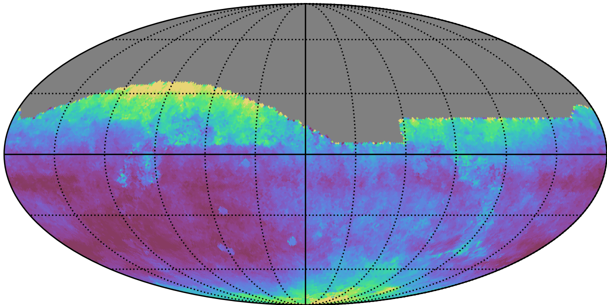
too_elab_r64_d3_giz_v3.4_10yrs All sky i band: Median seeingEff
