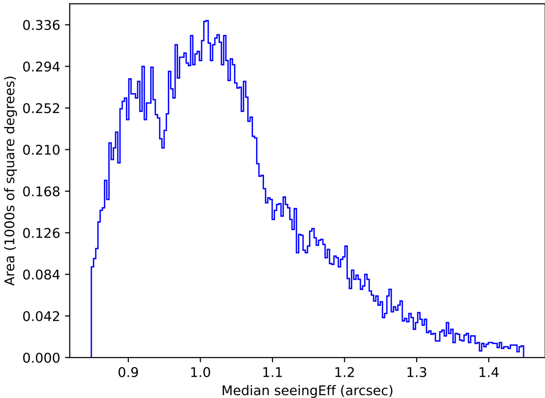
too_elab_r64_d3_giz_v3.4_10yrs All sky i band: Median seeingEff
