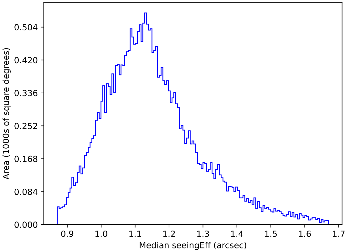
too_elab_r64_d3_giz_v3.4_10yrs All sky g band: Median seeingEff
