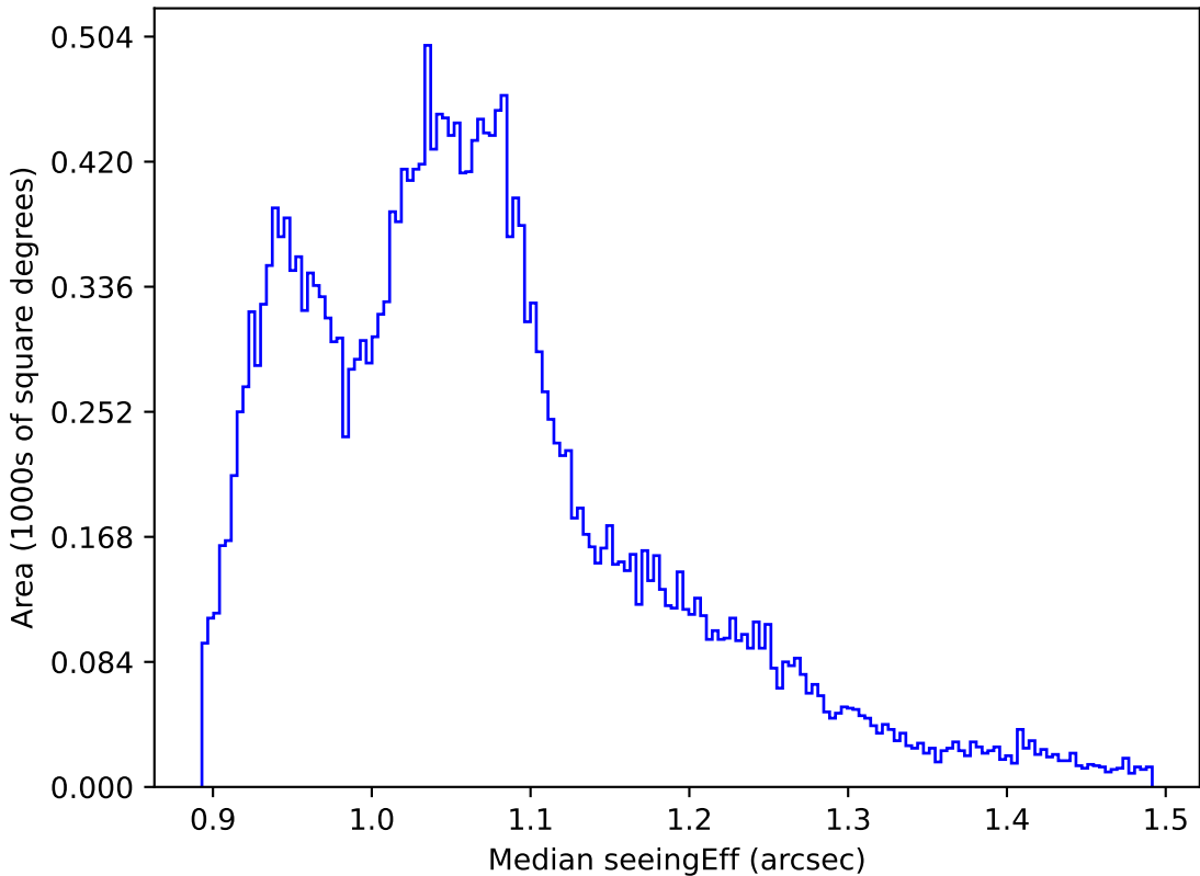
too_elab_r64_d3_giz_v3.4_10yrs All sky all bands: Median seeingEff
