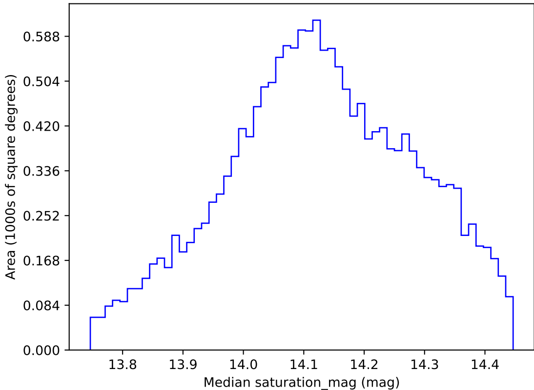
too_elab_r64_d3_giz_v3.4_10yrs WFD z band: Median saturation_mag
