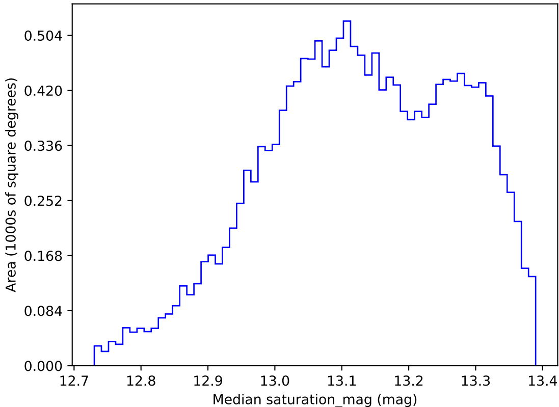
too_elab_r64_d3_giz_v3.4_10yrs WFD y band: Median saturation_mag
