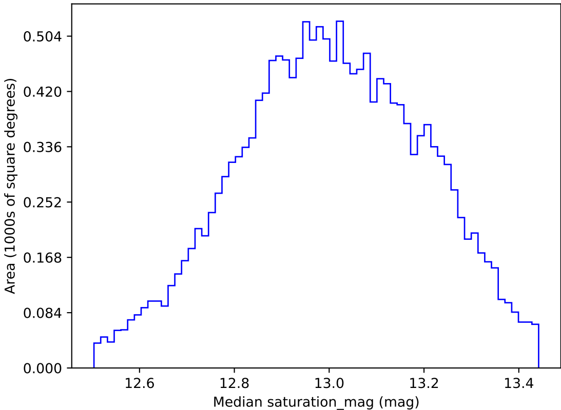
too_elab_r64_d3_giz_v3.4_10yrs WFD u band: Median saturation_mag
