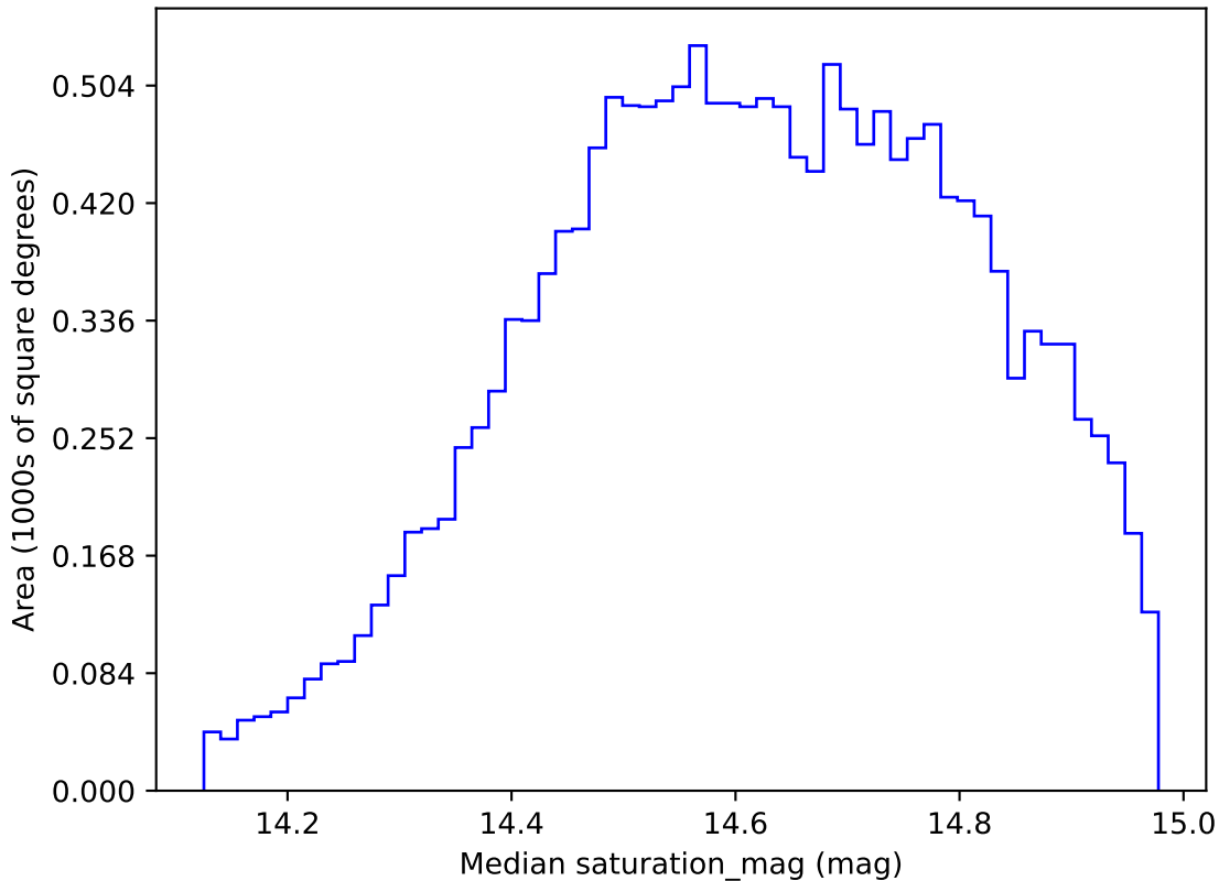
too_elab_r64_d3_giz_v3.4_10yrs WFD r band: Median saturation_mag
