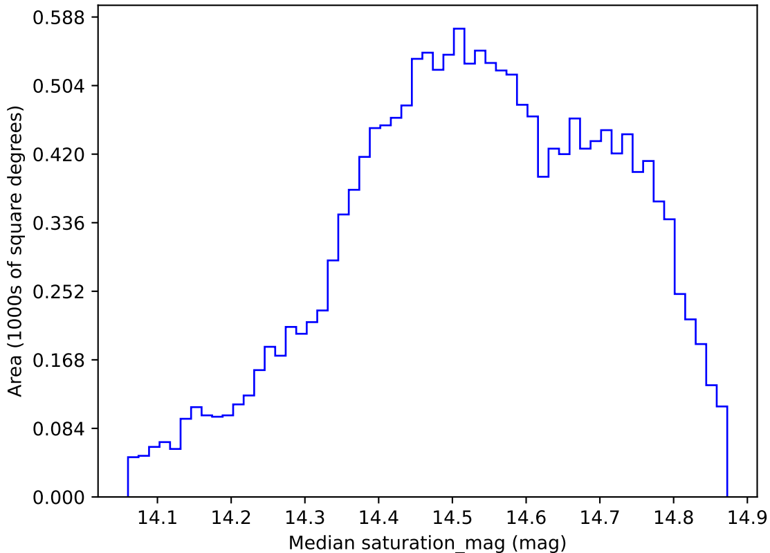
too_elab_r64_d3_giz_v3.4_10yrs WFD i band: Median saturation_mag
