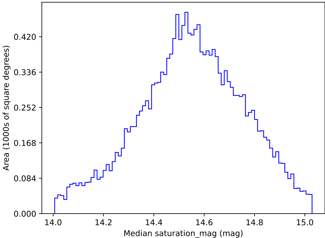
too_elab_r64_d3_giz_v3.4_10yrs WFD g band: Median saturation_mag
