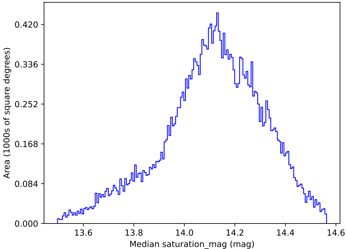
too_elab_r64_d3_giz_v3.4_10yrs All sky all bands: Median saturation_mag
