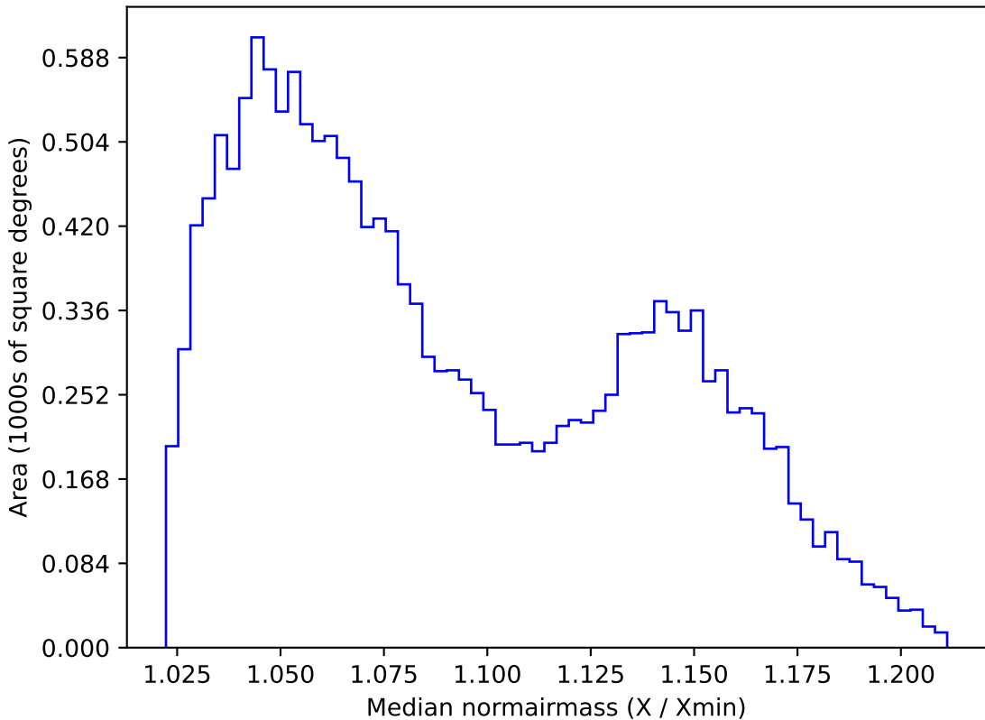
too_elab_r64_d3_giz_v3.4_10yrs WFD z band: Median normairmass
