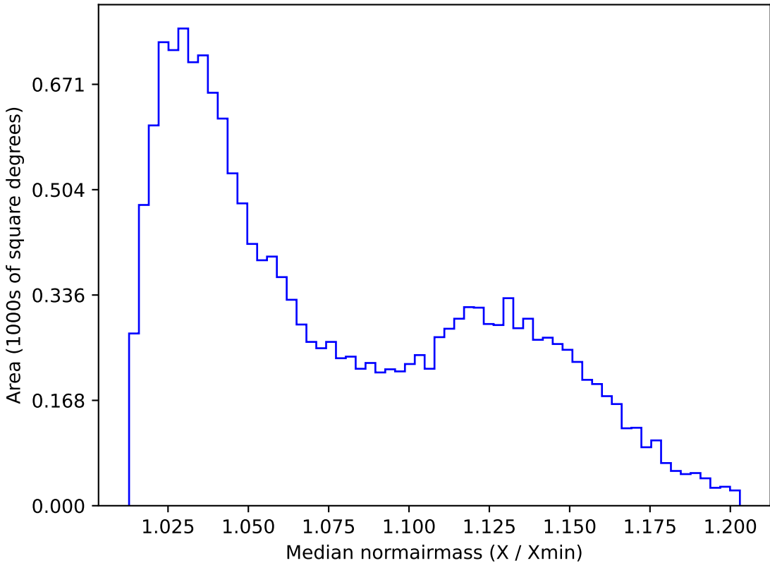
too_elab_r64_d3_giz_v3.4_10yrs WFD u band: Median normairmass
