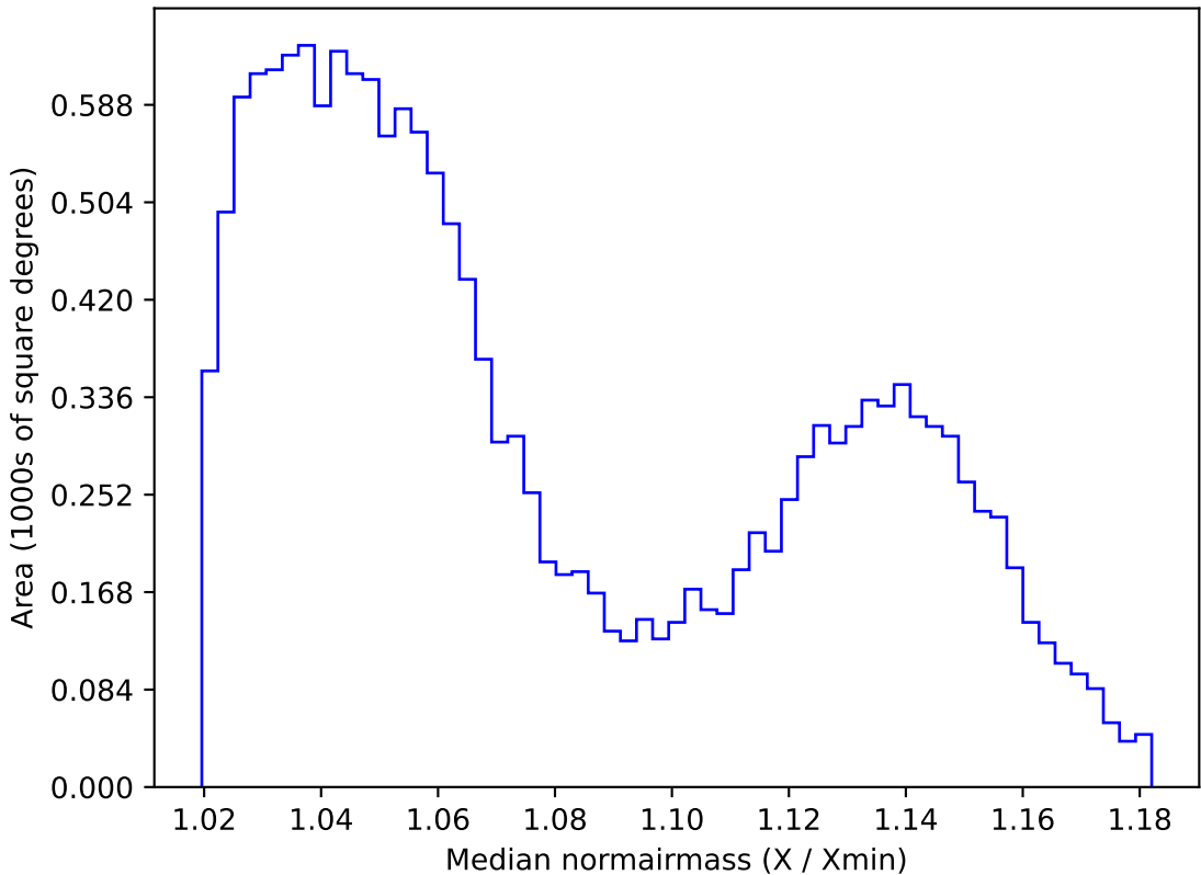
too_elab_r64_d3_giz_v3.4_10yrs WFD i band: Median normairmass
