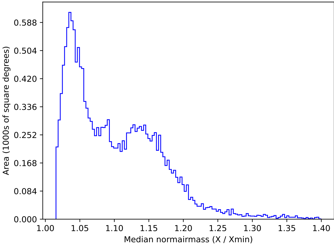
too_elab_r64_d3_giz_v3.4_10yrs WFD g band: Median normairmass
