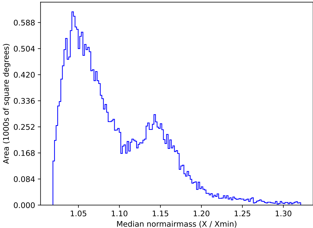
too_elab_r64_d3_giz_v3.4_10yrs All sky z band: Median normairmass
