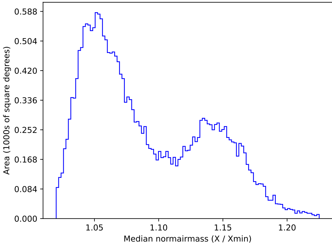
too_elab_r64_d3_giz_v3.4_10yrs All sky y band: Median normairmass
