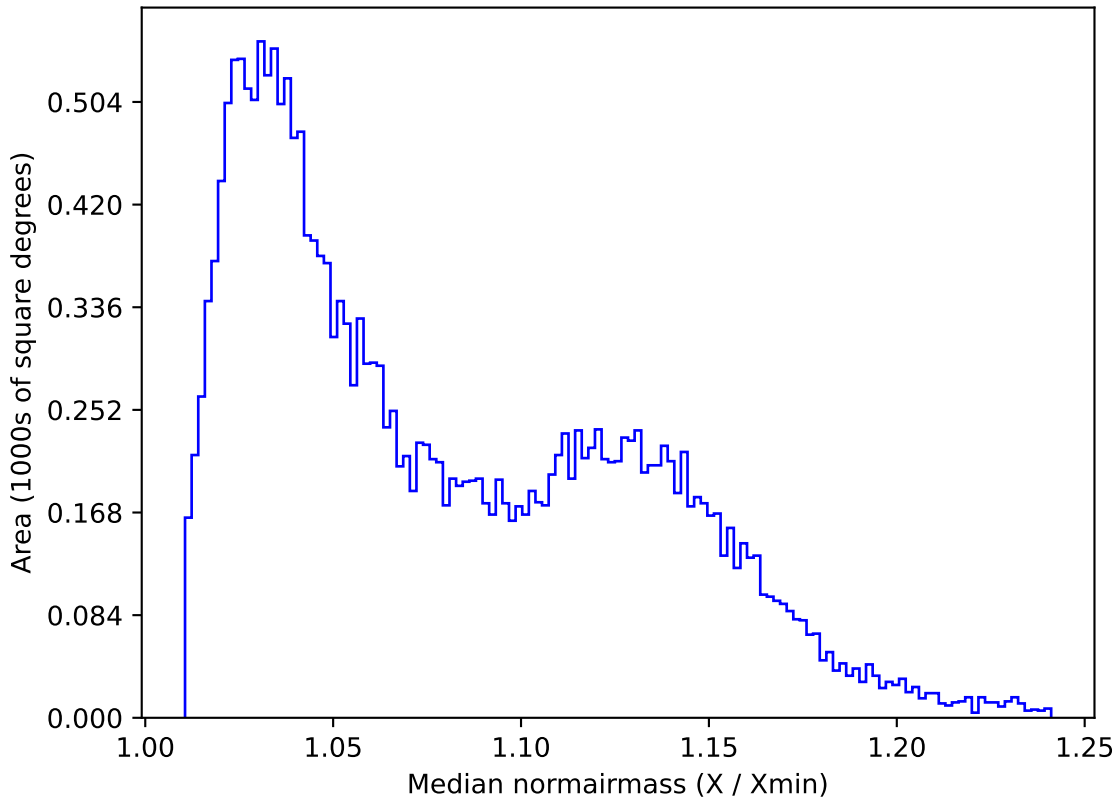
too_elab_r64_d3_giz_v3.4_10yrs All sky u band: Median normairmass
