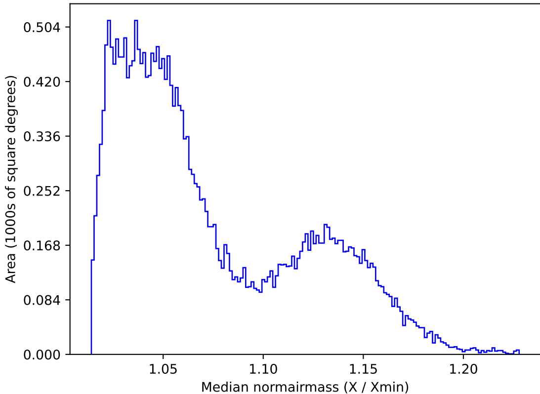
too_elab_r64_d3_giz_v3.4_10yrs All sky r band: Median normairmass
