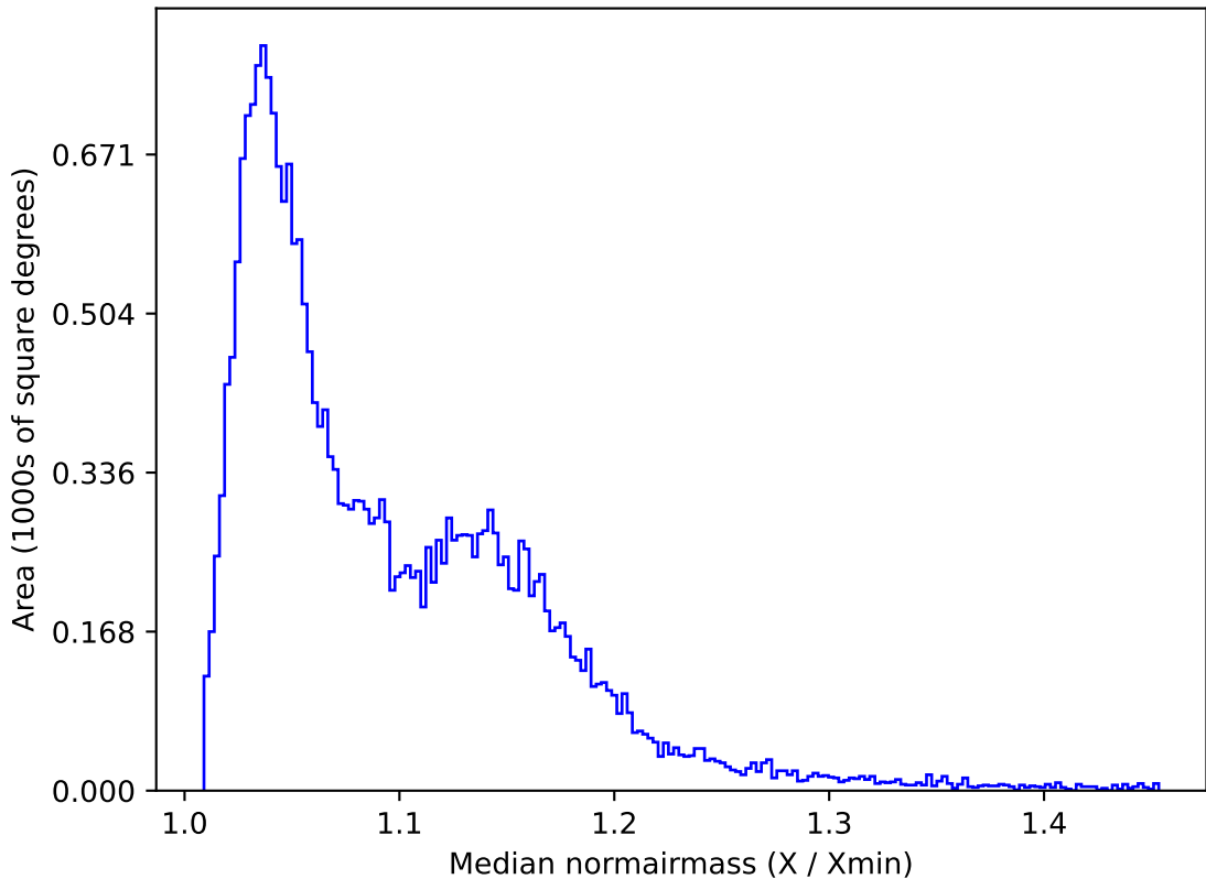
too_elab_r64_d3_giz_v3.4_10yrs All sky g band: Median normairmass
