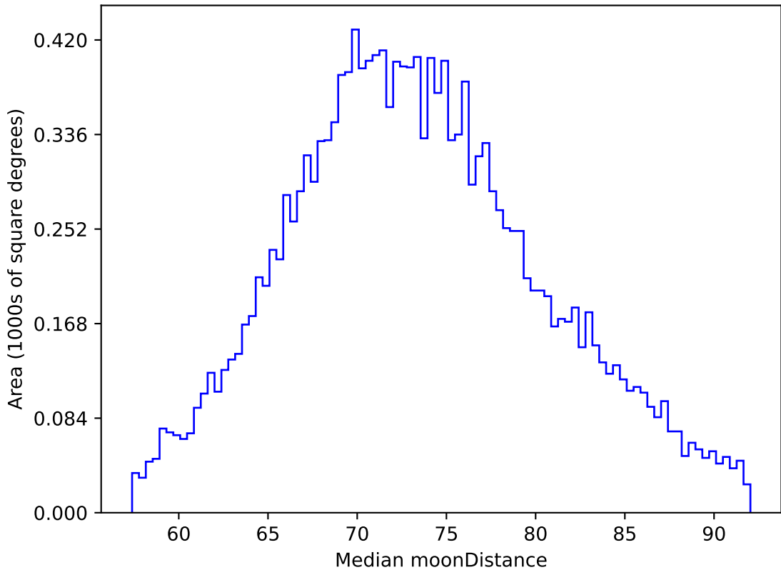
too_elab_r64_d3_giz_v3.4_10yrs WFD z band: Median moonDistance
