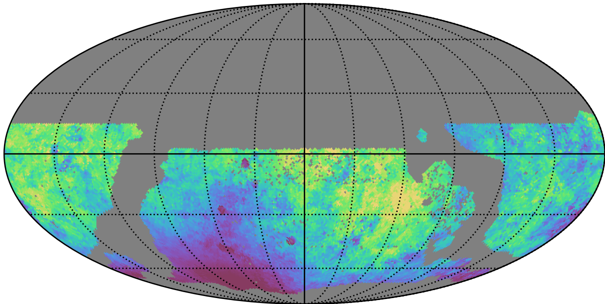
too_elab_r64_d3_giz_v3.4_10yrs WFD r band: Median moonDistance
