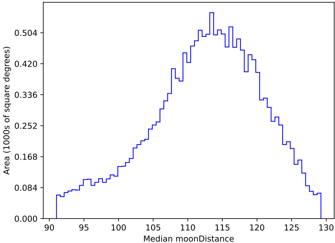
too_elab_r64_d3_giz_v3.4_10yrs WFD r band: Median moonDistance
