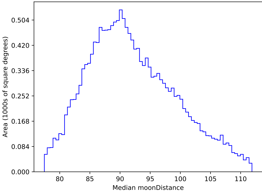
too_elab_r64_d3_giz_v3.4_10yrs WFD i band: Median moonDistance
