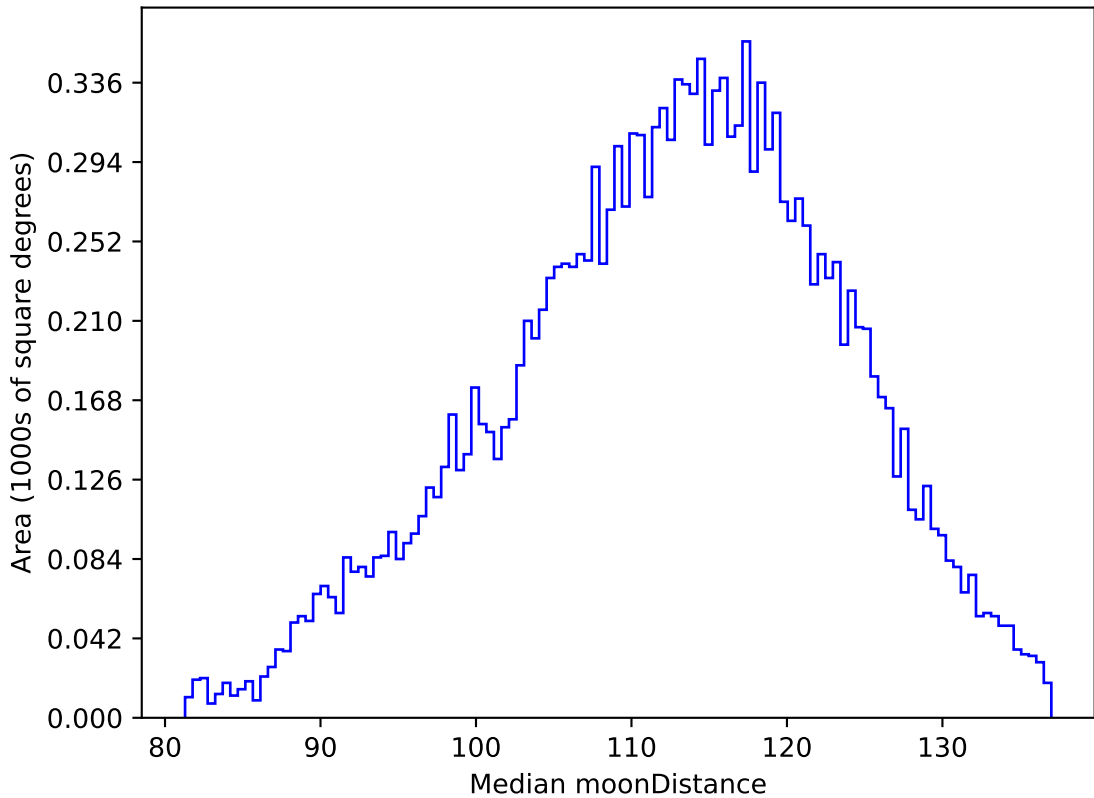
too_elab_r64_d3_giz_v3.4_10yrs WFD g band: Median moonDistance
