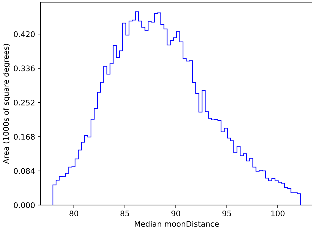
too_elab_r64_d3_giz_v3.4_10yrs WFD all bands: Median moonDistance
