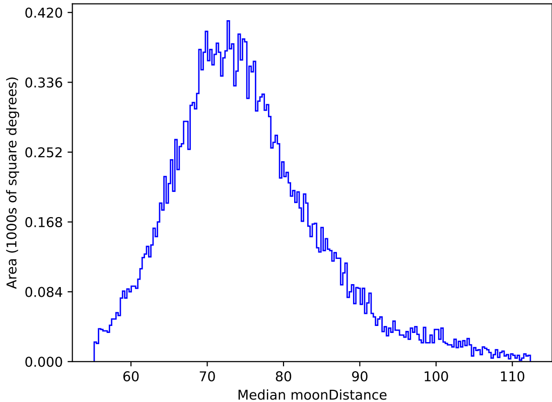
too_elab_r64_d3_giz_v3.4_10yrs All sky z band: Median moonDistance
