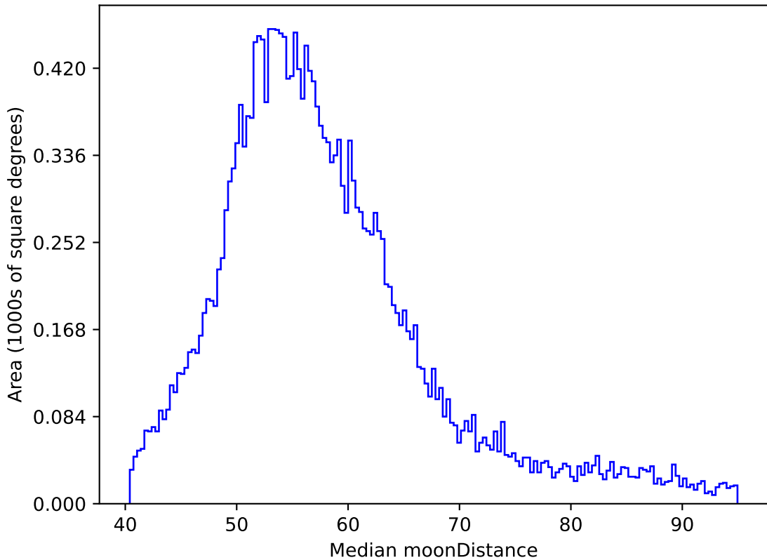
too_elab_r64_d3_giz_v3.4_10yrs All sky y band: Median moonDistance
