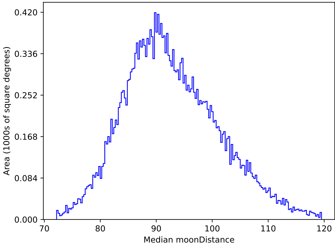
too_elab_r64_d3_giz_v3.4_10yrs All sky i band: Median moonDistance
