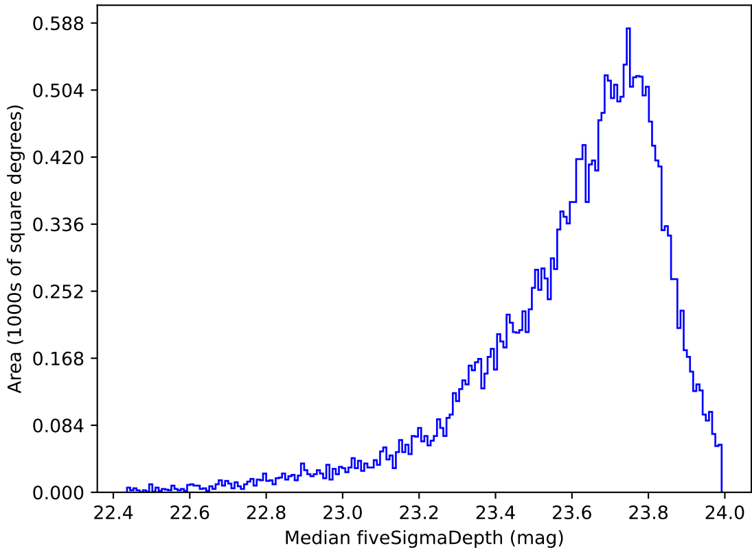
too_elab_r64_d3_giz_v3.4_10yrs Yr 1 i band: Median fiveSigmaDepth
