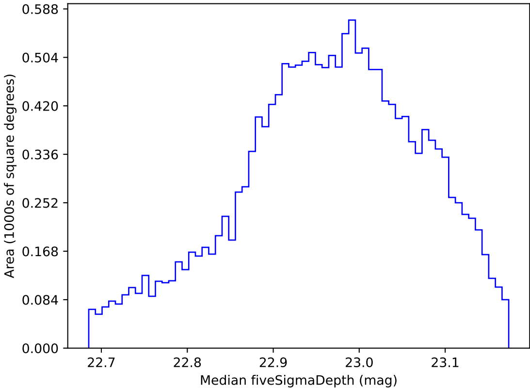
too_elab_r64_d3_giz_v3.4_10yrs WFD z band: Median fiveSigmaDepth
