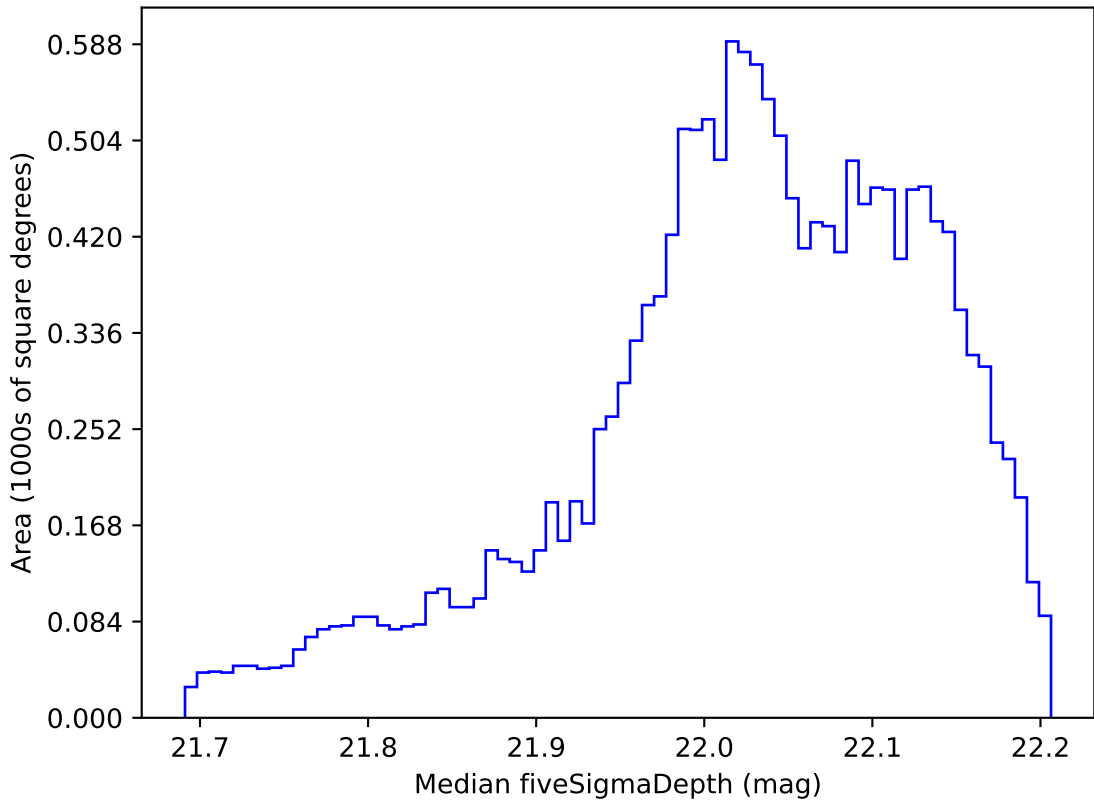
too_elab_r64_d3_giz_v3.4_10yrs WFD y band: Median fiveSigmaDepth
