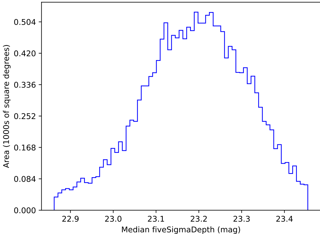
too_elab_r64_d3_giz_v3.4_10yrs WFD u band: Median fiveSigmaDepth
