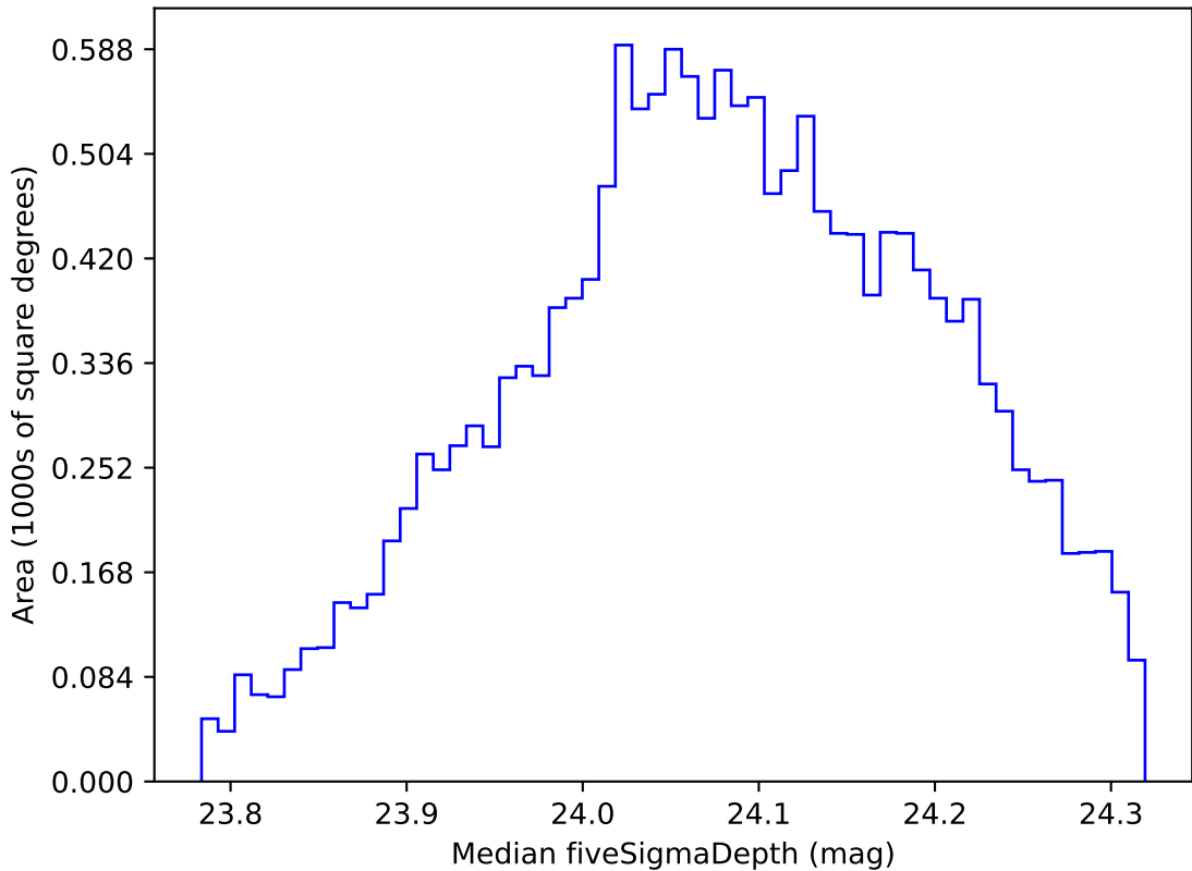
too_elab_r64_d3_giz_v3.4_10yrs WFD r band: Median fiveSigmaDepth
