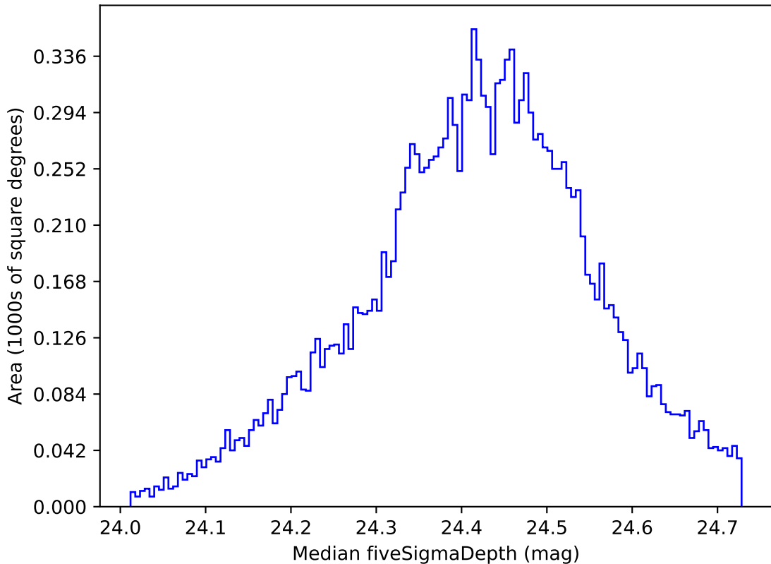
too_elab_r64_d3_giz_v3.4_10yrs WFD g band: Median fiveSigmaDepth
