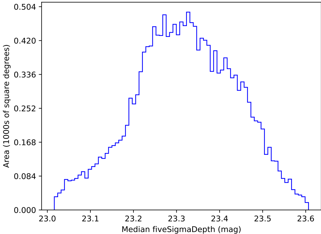
too_elab_r64_d3_giz_v3.4_10yrs WFD all bands: Median fiveSigmaDepth
