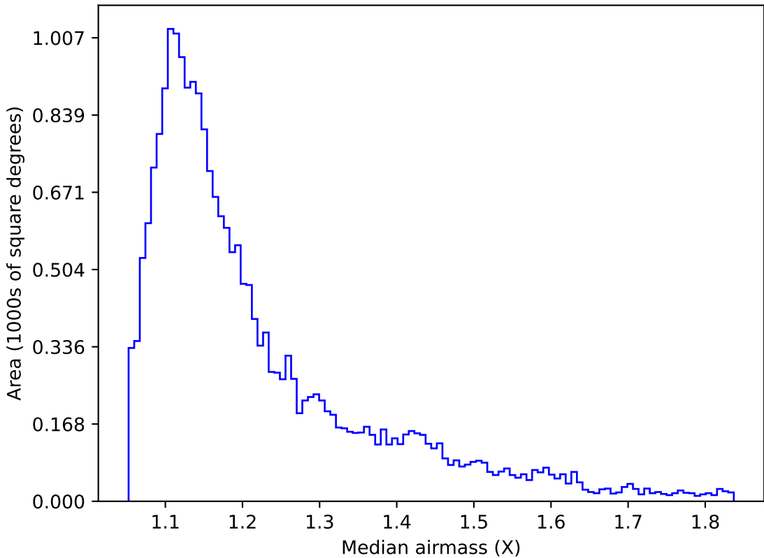
too_elab_r64_d3_giz_v3.4_10yrs Yr 1 u band: Median airmass
