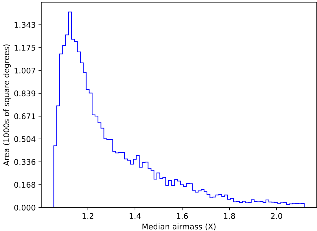
too_elab_r64_d3_giz_v3.4_10yrs Yr 1 g band: Median airmass
