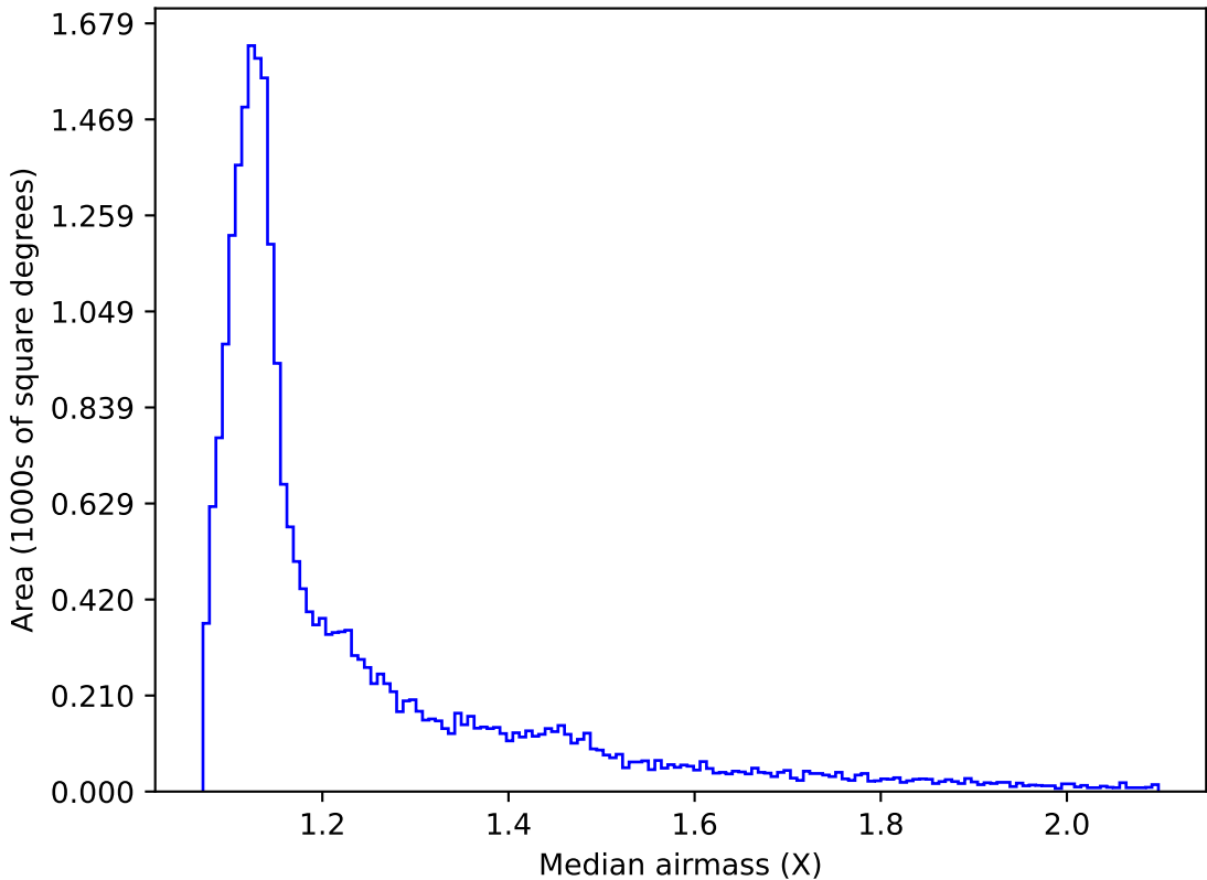
too_elab_r64_d3_giz_v3.4_10yrs Yr 1 all bands: Median airmass
